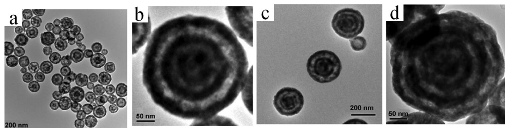
Fig. 20 TEM images of (a) double-shelled, (b) and (c) triple-shelled, and (d) quadruple-shelled \text{Cu}_2\text{O} hollow spheres for different CTAB concentrations: (a and b) 0.13 and (c and d) 0.15 M. Reprinted from ref. 75 with kind permission.
