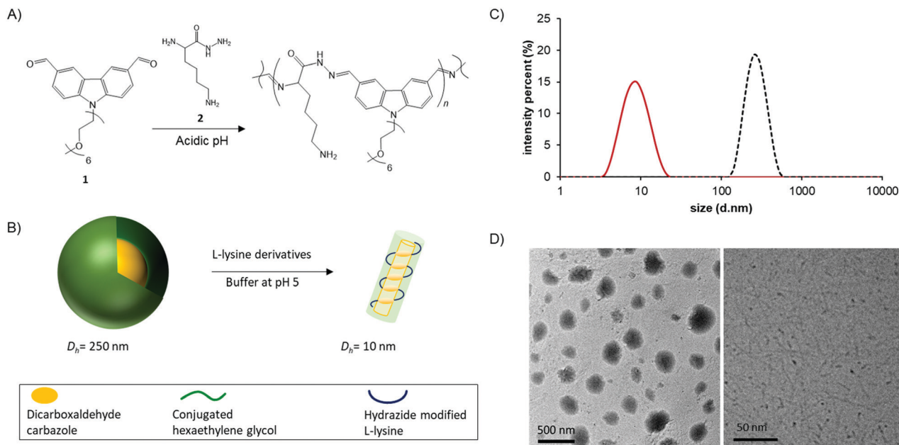
Fig. 1 Chemical structure of the monomers 1 and 2 and the corresponding molecular biodymymer (A) and illustration of carbazole-based dialdehyde 1 micelles ( D_h = 250 nm) transferring to biodymymer ( D_h = 10 nm) (B). Size of the carbazole micelle (dotted line, Z_{ave} = 255 nm, polydispersity index (PDI) = 0.077) and biodynamers (solid line, Z_{ave} = 8 nm, PDI = 0.099) obtained by DLS (C). TEM image of carbazole-based dialdehyde 1 micelles (D, left) and cryo-TEM image of biodynamers (D, right).
