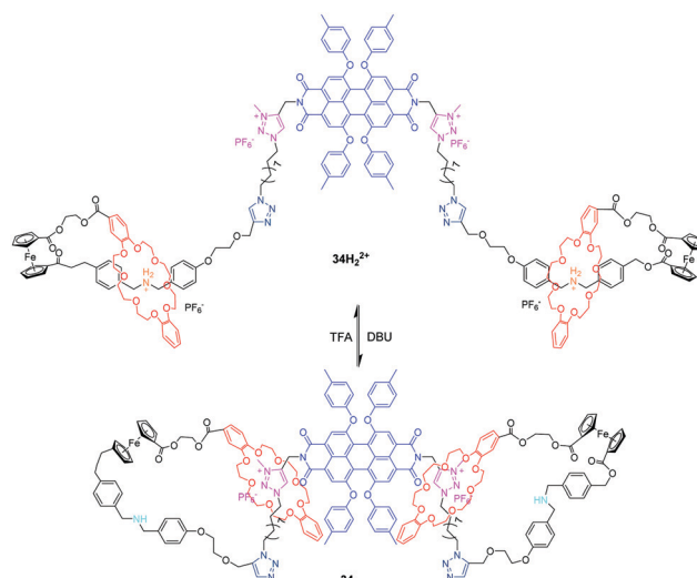
Fig. 34 pH-Controllable bis[1]rotaxane 34 .
