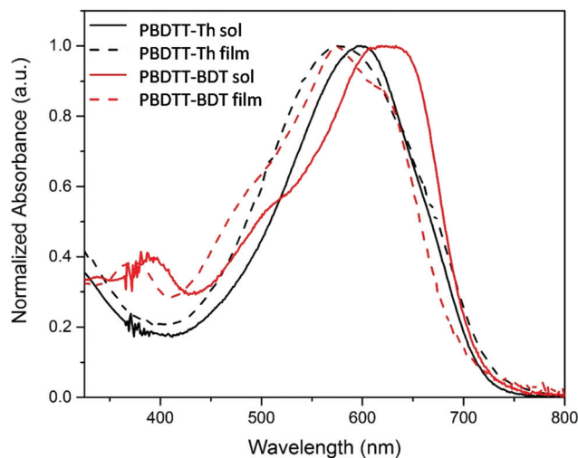
Fig. 3 Absorption spectra of polymers in solution ( \text{CHCl}_3 , solid lines) and thin film (cast from \text{CHCl}_3 , dashed lines).
