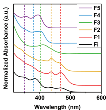
Fig. 4 Absorption spectra for the fraction obtained by size selective precipitation from the reaction mixture at 350 \text{ }^\circ\text{C} and 4.5 \text{ s} . The table shows the absorption maxima of the CdSe species, their diameters and the calculated aggregation numbers. Fi is the initial sample and F1, ..., F5 the consecutive fractions obtained.
