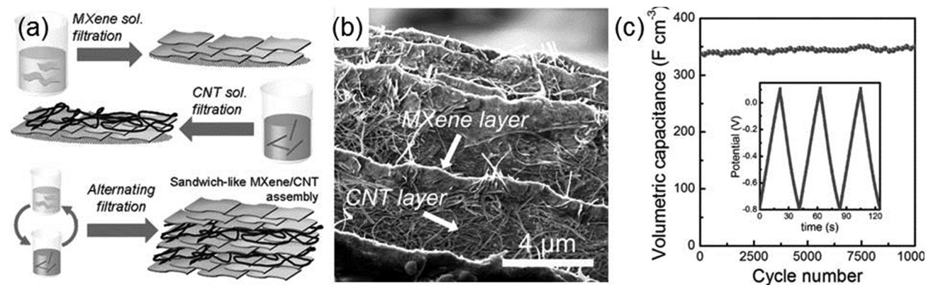
Fig. 7 (a) Preparation of the sandwich-like \text{Ti}_3\text{C}_2\text{T}_x\text{-CNT} composite. (b) Cross-sectional SEM images of \text{Ti}_3\text{C}_2\text{T}_x\text{-CNT} papers. (c) Cycling stability of the \text{Ti}_3\text{C}_2\text{T}_x\text{-CNT} electrode at 10\text{ A g}^{-1} . Reprinted with permission from ref. 92 Copyright (2015) Wiley Online Library.
