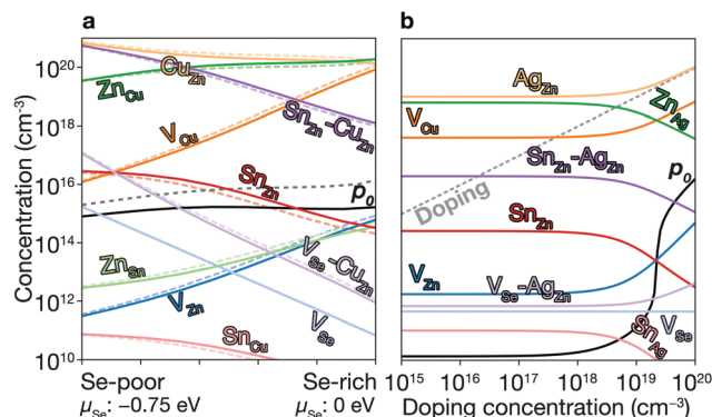
Fig. 6 Concentrations of native defects. (a) The concentrations of native defects in \text{CZTSe} . The dashed lines represent the concentration with the doping during the growth (see text for details). (b) The concentrations of native defects in \text{AZTSe} with the doping during the growth. The dashed diagonal line represents the doping concentration.
