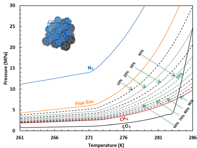
Fig. 5 Hydrate stability zones of CO 2 , N 2 , CH 4 , flue gas (14.6% CO 2 and 85.4% N 2 ) and mixtures of flue gas with CH 4 (dotted lines) as a function of temperature. Increasing the pressure of the system above the predicated phase boundaries could initiate the hydrate formation. Adding gases with higher hydrate stability pressure zones to gases with lower hydrate stability pressure zones, shifts the system phase boundaries to the left (adapted with permission from Hassanpouryouzband et al. , 81 Copyright 2019 Springer Nature).
