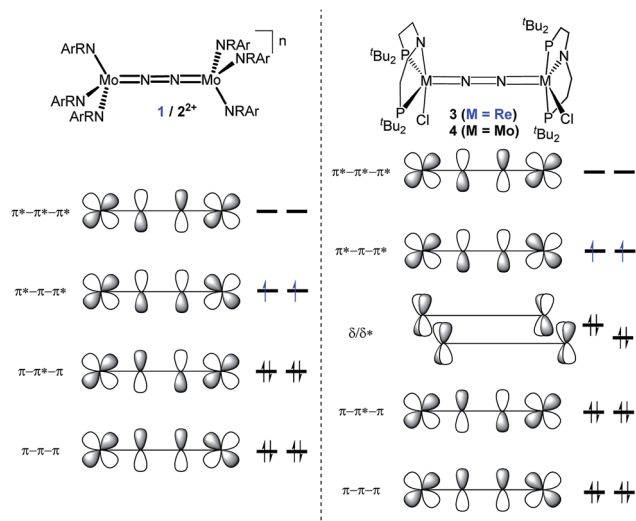
Fig. 1 Qualitative molecular orbital schemes for 1, 2^{2+} , 3 and 4, illustrating the isolobal relationship of 1 \{\pi^{10}\} /3 \{\pi^{10}\delta^4\} and 2^{2+} \{\pi^8\} /4 \{\pi^8\delta^4\} , respectively.
