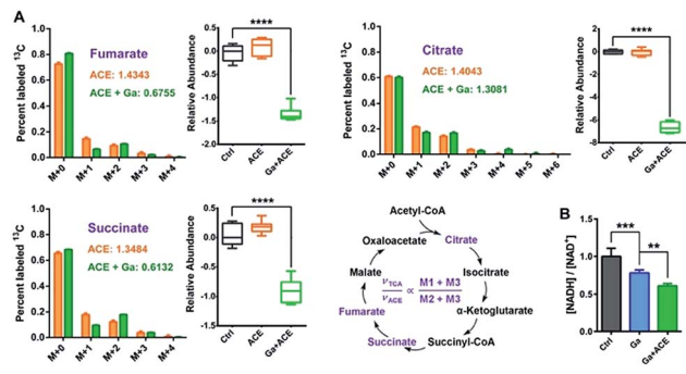
Fig. 5 Combined Ga(III) and acetate treatment leads to reduced TCA cycle flow. (A) Mass isotopomer distributions of ^{13}\text{C}_2 -labelled acetate detected in the TCA cycle and the relative abundances of cycle metabolites. (B) Ratios of bacterial cellular NADH and \text{NAD}^+ levels after treatment with Ga(III) and acetate. Data are presented as mean \pm SEM from biological replicates. The asterisks indicate significant difference from the Ctrl or Ga(III) treatment group (*, 0.001 < p < 0.01 and ***, p < 0.001 ).
