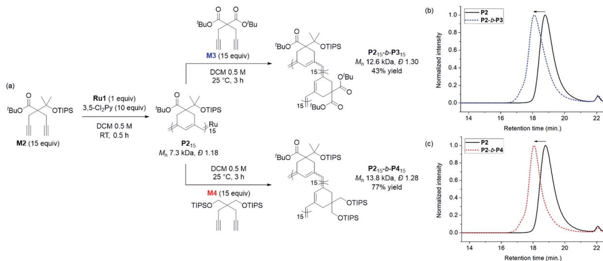
Scheme 2 (a) Diblock copolymerization of with M2 as the first monomer, and M3 (above) and M4 (below) as the second monomers. SEC traces of homopolymer P2 and diblock copolymers: (b) P2-b-P3, and (c) P2-b-P4.
