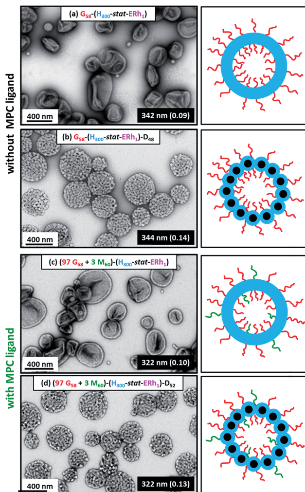
Fig. 3 Representative TEM images (and corresponding hydrodynamic diameters and DLS polydispersities) obtained for fluorescently-labeled (a) smooth G_{58}\text{-(H}_{300}\text{-stat-ERh}_1) diblock copolymer vesicles, (b) framboidal G_{58}\text{-(H}_{300}\text{-stat-ERh}_1)\text{-D}_{48} triblock copolymer vesicles, (c) smooth (97 G_{58} + 3 M_{60})\text{-(H}_{300}\text{-stat-ERh}_1) diblock copolymer vesicles and (d) framboidal (97 G_{58} + 3 M_{60})\text{-(H}_{300}\text{-stat-ERh}_1)\text{-D}_{52} triblock copolymer vesicles synthesized at pH 7.4 under sterile conditions. Corresponding color-coded schematic cartoons are also shown for each type of vesicle.
