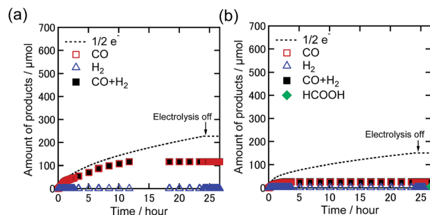
Fig. 6 Time courses of the generation of CO (red square), \text{H}_2 (blue triangle), sum of CO and \text{H}_2 (black-filled square), and formic acid (green diamond) during bulk electrolysis using Re-DMF + (0.5 mM) at -1.82 V in a DMF solution containing \text{Et}_4\text{NBF}_4 (0.1 M) under (a) 100% and (b) 1% \text{CO}_2 atmospheres ( 10 \text{ mL min}^{-1} ). Corresponding time courses of the current during bulk electrolysis are shown in Fig. S5.†
