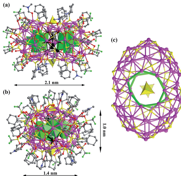
Fig. 1 (a) and (b) The X-ray crystal structure of \text{Ag}_{10}@\text{(Mo}_7\text{O}_{26})_2@\text{Ag}_{70} nanoclusters viewed along two orthogonal directions. The inner silver atoms of the \text{Ag}_{10} kernel are highlighted in black. \text{Mo}_7\text{O}_{26}^{10-} and \text{MoO}_4^{2-} are represented by green and yellow polyhedra, respectively. (c) The \text{Ag}_{70}\text{S}_{36} shell with silver heptagons highlighted in green.
