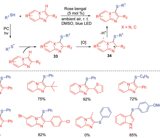
Scheme 16 Regioselective sulfenylation of imidazopyridines.
