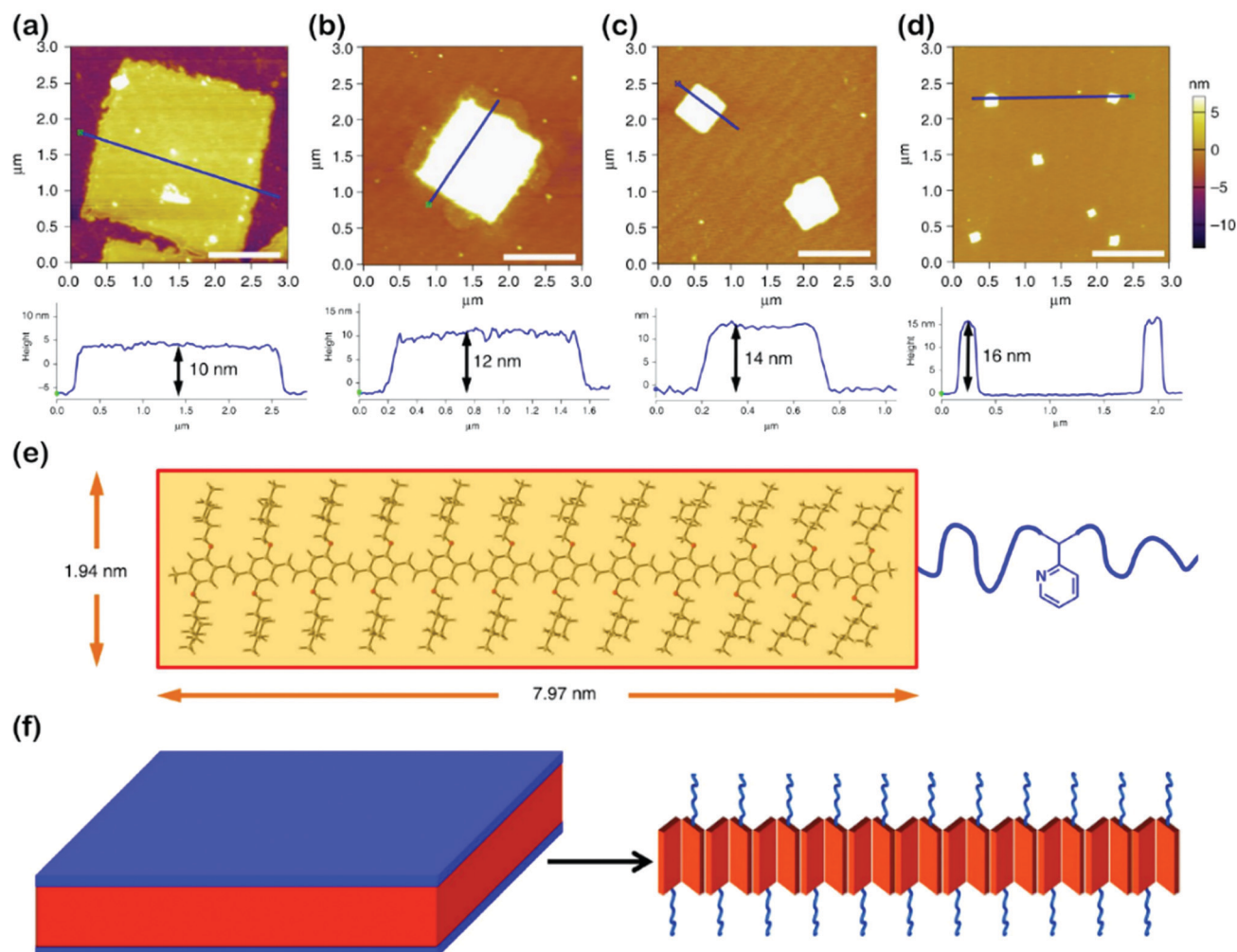
Fig. 9 (a–d) AFM height images of 2D square micelles with different dimensions, obtained from 2-PrOH solution of PPV 12 - b -P2VP 12 (a), PPV 12 - b -P2VP 22 (b), PPV 12 - b -P2VP 22 (c), and PPV 12 - b -P2VP 36 (d). Scale bars represent 1 \mu m. (e) The optimized molecular structure and calculated scales of the PPV 12 block by DFT calculations. (f) Schematic illustration and possible molecular packing of the square micelles. Reproduced with permission from ref. 61. Copyright 2018, Springer Nature.
