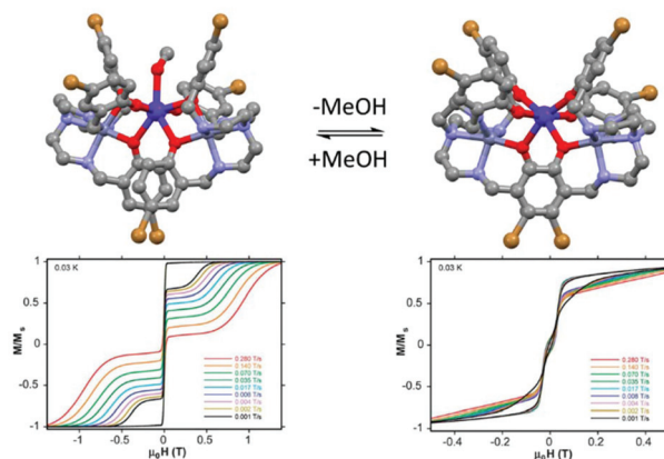
Fig. 10 Molecular structures of ( 24 ) (MeOH)·3MeOH with its hysteresis loop at 0.03 K (left part) and its methanol free analogue ( 24 ) with its hysteresis loop at 0.03 K (right part). Colour code: bromide: brown. Adapted from ref. 73.
