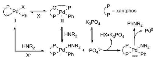
Fig. 8 Proposed mechanism of dehydrohalogenation and amide coordination in Pd-catalysed amide N -arylation. 89 Reprinted with permission. Copyright 2017 American Chemical Society.
