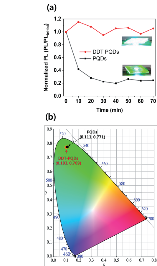
Fig. 5 (a) Change of the PL emissions and photographs (inset) of the PQDs (down) and DDT-PQDs (up) with respect to LED working time. (b) CIE color coordinates of LEDs.
