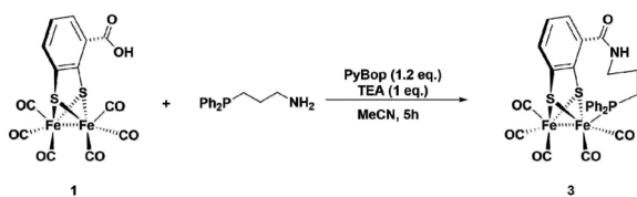
Fig. 3 One-pot synthesis of the propyl-tethered complex 3 . Complexes 4 was prepared in a similar fashion.
