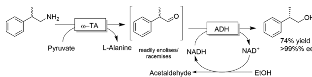
Scheme 28 Deracemisation of ( R,S )-2-phenylpropylamine to afford ( S )-2-phenylpropanol using a non-stereoselective \omega -TA coupled with an enantioselective ADH. The two steps were DEAR separately in a continuous flow system operating with a self-sustaining closed-loop.
