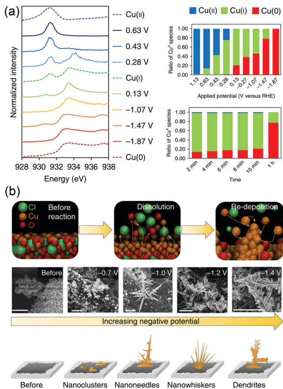
Fig. 21 (a) In situ Cu L 3 -edge X-ray spectra of electro-redeposited Cu at different applied potentials and references for Cu metal, Cu 2 O, and Cu 2 O. On the right side, calculated ratios of Cu oxidation states from linear combination fitting as a function of the applied potential or time. (b) Schematic representation of the growth of these nanostructures following simultaneous dissolution and redeposition of Cu. Representative SEM images (scale bars = 5 μm) collected at specific applied potentials after at least one hour of reaction. At -1.0 V RHE , sharp needles of 5 to 10 μm in length could be witnessed, whereas at -1.2 V RHE , sharp nanowhiskers of 5 to 10 μm with high length-to-diameter ratios predominated. At the most negative applied potential (-1.4 V RHE ), dendrites with rounded tips were reported. Adapted with permission from ref. 320. Copyright 2018 Springer Nature.
