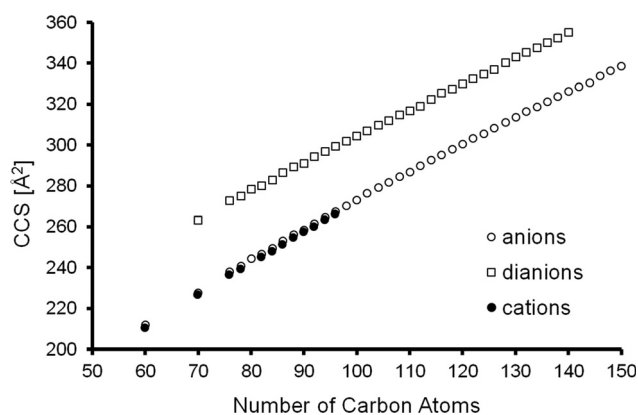
Fig. 2 Experimental {}^{\text{TIMS}}\text{CCS}_{\text{N}_2} of fullerene ions in the size range between 60 and 150 atoms (in three different charge states as indicated). The standard deviation is ca. 0.5% or 1 \text{ \AA}^2 which corresponds to the size of the symbols.
