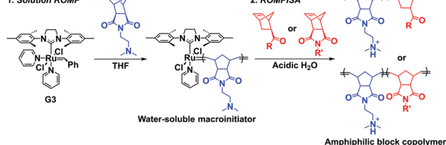
Scheme 2 Reported synthetic strategies to conduct aqueous dispersion ROMPISA for fabrication of diblock copolymer nano-objects of various morphologies. (A) One-pot aqueous ROMPISA mediated by a water-soluble HG2 catalyst, and (B) two-step aqueous ROMPISA mediated via a water-soluble PNB macroinitiator prepared in organic solvent using G3 .
