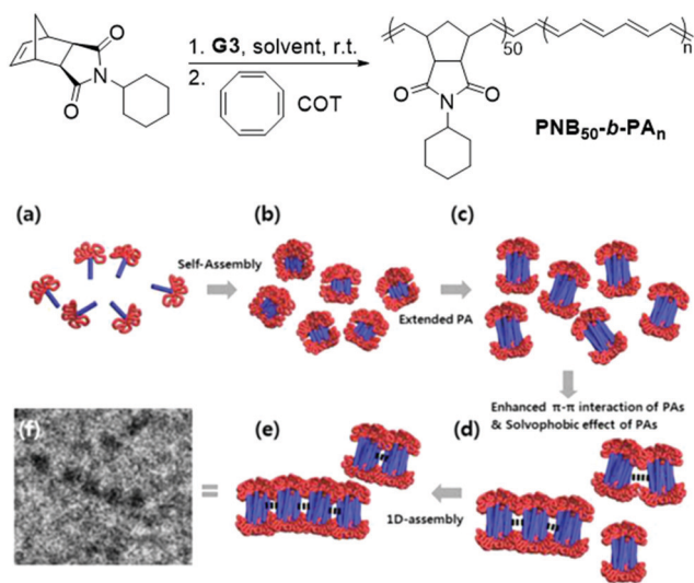
Fig. 1 Preparation of \text{PNB}_{50}\text{-}b\text{-PA}_n diblock copolymer “nanocaterpillars” via a one-pot ROMPIISA process and proposed 1D self-assembly mechanism. Adapted with permission from ref. 37. Copyright 2012 American Chemical Society.
