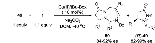
Scheme 22 Cu(II)-Catalyzed asymmetric 1,3-dipolar [4+3] cycloaddition and kinetic resolution of azoalkenes with azomethine imines.
