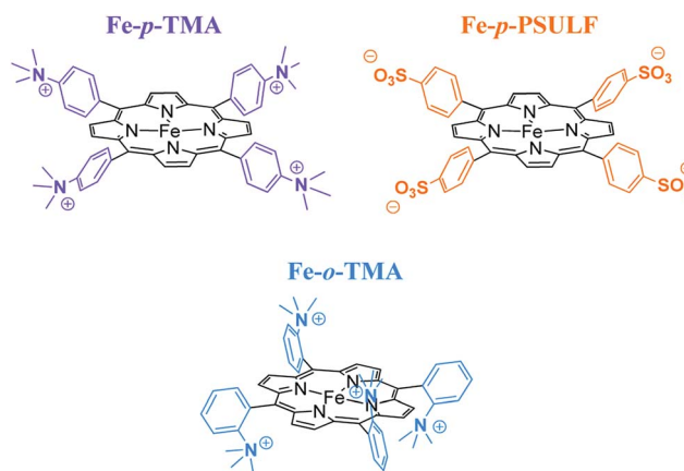
Fig. 2 Iron tetraphenylporphyrin derivatives with positive and negative charges used for electrocatalytic reduction of \text{CO}_2 to \text{CO} . Reprinted with permission from ref. 88. Copyright 2016, American Chemical Society.
