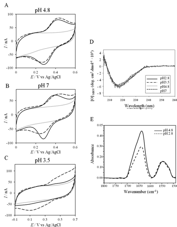
Fig. 3 (A–C) CVs of 50 μM AcoP at a PG electrode in the membrane configuration at pH 4.8 (A), pH 7 (B), and pH 3.5 (C) in 20 mM \text{NH}_4\text{AC} buffer, before (black solid lines) and after the addition of 200 mM NaCl (black dashed line). v = 20 \text{ mV s}^{-1} . Grey solid lines represent the CVs with no protein; (D) CD spectra of AcoP at different pHs in 10 mM \text{NH}_4\text{AC} buffer at room temperature; (E) ATR-FTIR spectra of AcoP at 20 μM in 10 mM \text{NH}_4\text{AC} at pH 4.8 (solid line) and pH 2.8 (dashed line).
