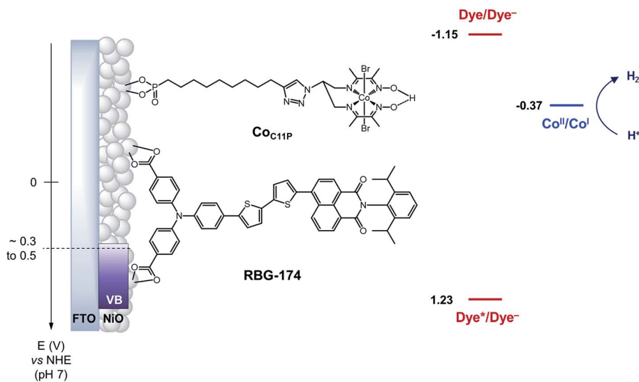
Fig. 1 Schematic energy diagram of the NiOIRBG-174| \text{CoC}_{11}\text{P} photocathode. See text for the estimation of energy levels at pH = 7. Potentials for the redox couples of RBG-174 have been determined as described in ref. 48 from data found in ref. 40.
