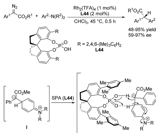
Scheme 32 Catalytic asymmetric arylation of \alpha -aryl- \alpha -diazoacetates with aniline derivatives.
