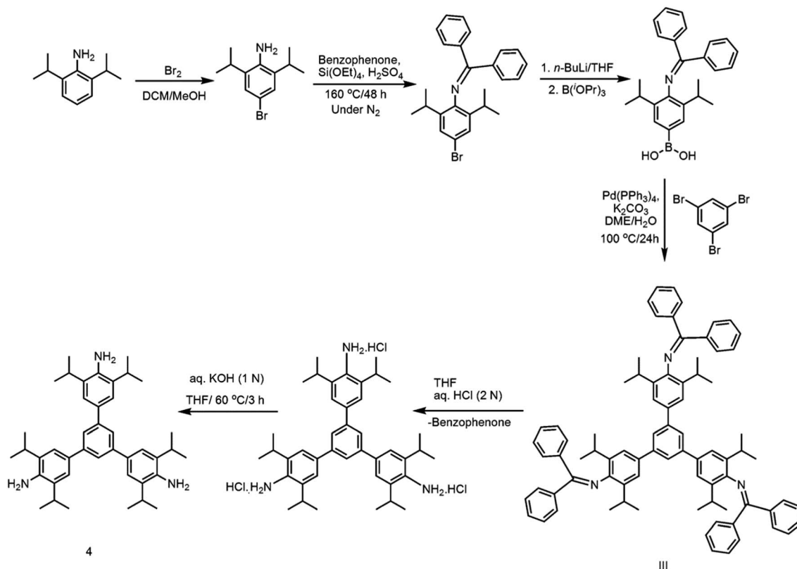
Scheme 3 Synthesis of 4 .
