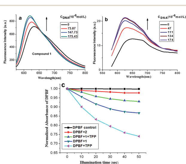
Fig. 2 Fluorescence spectra of compound 1 (a) and 2 (b) with the titration to ct-DNA. Each spectrum was recorded in pH = 7.4, 0.05 \text{ mol L}^{-1} Tris-HCl, 0.1 \text{ mol L}^{-1} NaCl buffer solution. (c) Singlet oxygen generation of 1 and 2 ( 50 \mu\text{M} ). The change of absorption of DPBF at 418 nm ( A/A_0 ) upon the irradiation time. The spectrum was recorded in DMSO.
