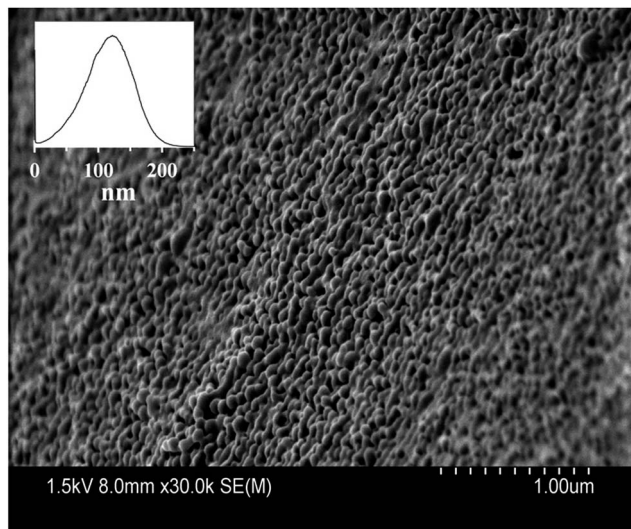
Fig. 4 Scanning electron micrograph of blank-PLGA nanoparticles. The insert represents the particle size distribution histogram of blank-PLGA nanoparticles.
