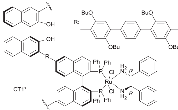
Scheme 14 Sequential enantioselective Et 2 Zn addition – enantioselective hydrogenation by a chiral copolymer immobilized R,R -32-Ru-complex. 130
