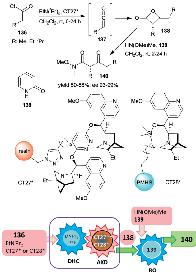
Scheme 40 One-pot acid chloride dehydrochlorination (DHC) and asymmetric ketene dimerization (AKD) using heterogeneous cinchona alkaloid catalyst followed by ring opening (RO) to Weinreb amides; PMHS: poly(methylhydrosiloxane). 185,186
