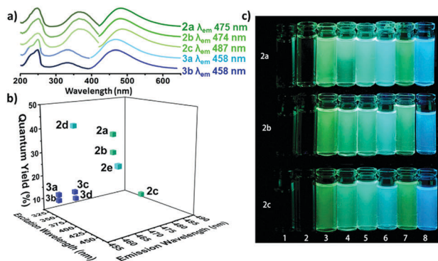
Fig. 1 (a) UV and emission spectra of fluorescent aminomaleimides ( 2a–c ) and alkoxybromomaleimides ( 3a–e ); (b) fluorescence quantum yields of the singly substituted maleimides ( 2a–e , 3a–d ) against excitation and emission wavelengths (recorded at 10 \mu M in diethyl ether); (c) aminomaleimides ( 2a–c ) in 8 solvents (1–8: H 2 O, MeOH, DMF, dioxane, THF, Et 2 O, CH 2 Cl 2 and cyclohexane) under UV light (365 nm).
