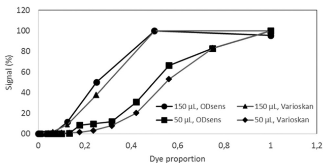
Fig. 4 Validation of the OD sensor – comparison with a Varioskan(R) instrument in 150 and 50 \mu\text{L} of sample dilutions of the green food dye (E143), N = 3 .
