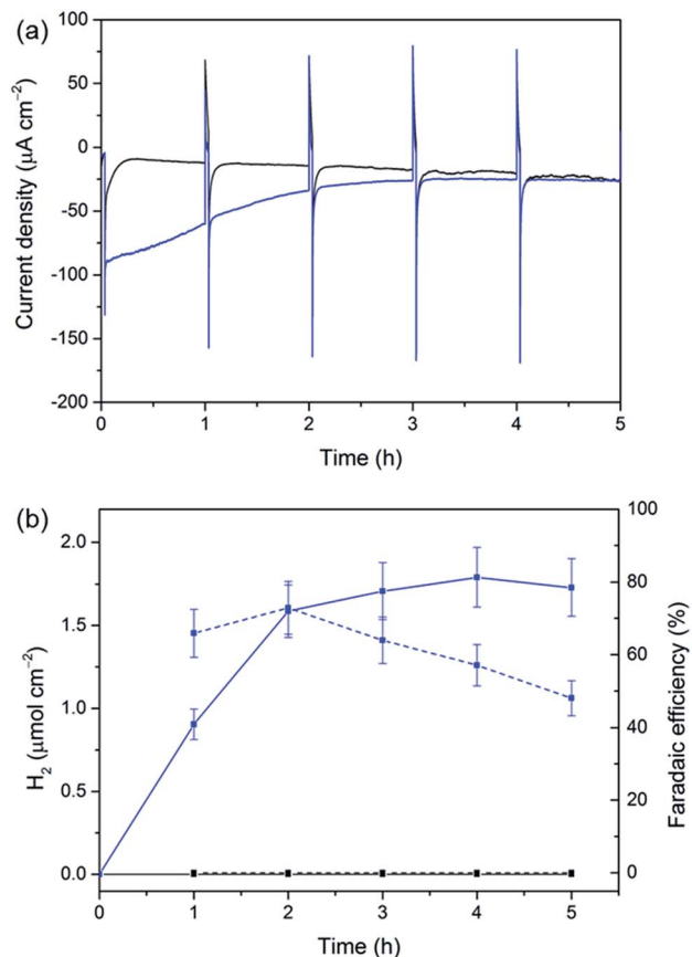
Fig. 5 CPP traces for \text{Si|mesoTiO}_2 (black) and \text{Si|mesoTiO}_2|\text{H}_2\text{ase} (blue) at 0.0 V vs. RHE during continuous illumination with UV-filtered simulated solar light (AM1.5G, 100 \text{ mW cm}^{-2} , \lambda > 400 \text{ nm} ). (a) Chronoamperograms with an hourly dark chop lasting for two min each and (b) \text{H}_2 evolution (solid traces) and cumulative faradaic efficiency (dashed traces). Conditions: aqueous 2-( N -morpholino)ethanesulphonic acid solution (50 mM, pH 6), inert atmosphere, room temperature.
