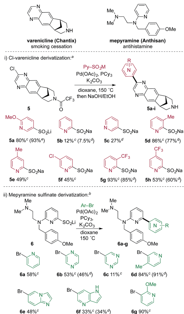
Scheme 2 Application of pyridine sulfinate coupling reaction to medicinal chemistry targets. a Reaction conditions for varenicline library: 0.10 mmol scale, varenicline-Cl (1.0 equiv.), sulfinate (2.0 equiv.), Pd(OAc) 2 (5 mol%), PCy 3 (7.5 mol%), K 2 CO 3 (2.0 equiv.), 12 h in a sealed 0.5–2 mL microwave vial in a 150 °C aluminum block; then, in the same pot, 1.0 M aq. NaOH and EtOH and heated at 50 °C for 1 h. b Reaction conditions for mepyramine library: 0.083 mmol scale, Het-Br (1.0 equiv.), sulfinate core (1.2 equiv.), Pd(OAc) 2 (5 mol%), PCy 3 (7.5 mol%), K 2 CO 3 (2 equiv.), 12 h in a sealed 0.5–2 mL microwave vial in a 150 °C aluminum block. c Yield after automated HPLC purification. d NMR yield based on analysis of the crude product prior to purification. e Yield from an isolated single experiment.
