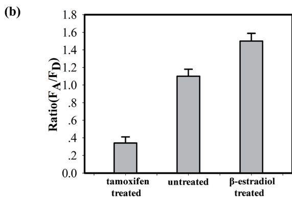
Fig. 5 (a) Fluorescence imaging of TK1 mRNA in HepG2 cells (tamoxifen treated, untreated and β-estradiol treated) by MnO 2 nanosheet mediated “DD–A” FRET binary probes. (b) The histogram of the relative fluorescence intensity (A/D) of the above three groups. The excitation wavelength is 488 nm, and the images were collected in the range of 505–560 nm (FAM) and >560 nm (TAMRA). Scale bar: 10 μm.
