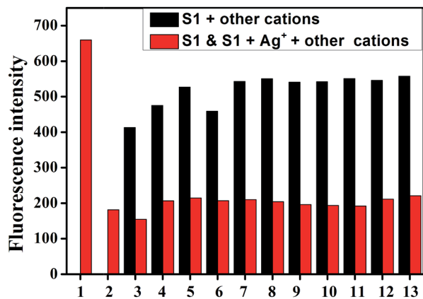
Fig. 2 Fluorescent emission ( \lambda_{\text{ex}} = 400 \text{ nm} ) spectra of S1 ( 2 \times 10^{-5} \text{ M} ) and Ag + (10 equiv.) in the presence of various competing cations in DMSO/H 2 O (v:v = 1 : 1, buffered with HEPES pH = 7.2) solution. From 1 to 13: S1, S1 + Ag + , S1 + Ag + + Fe 3+ , S1 + Ag + + Ca 2+ , S1 + Ag + + Cu 2+ , S1 + Ag + + Co 2+ , S1 + Ag + + Ni 2+ , S1 + Ag + + Cd 2+ , S1 + Ag + + Pb 2+ , S1 + Ag + + Zn 2+ , S1 + Ag + + Hg 2+ , S1 + Ag + + Cr 3+ , and S1 + Ag + + Mg 2+ , respectively.
