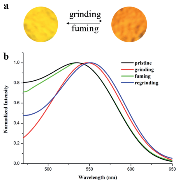
Fig. 4 (a) Photos of TBM changes under grinding and fuming stimuli; (b) normalized fluorescence spectra of TBM in different solid-states: pristine, grinding, fuming and regrinding, \lambda_{ex} = 410 nm.
