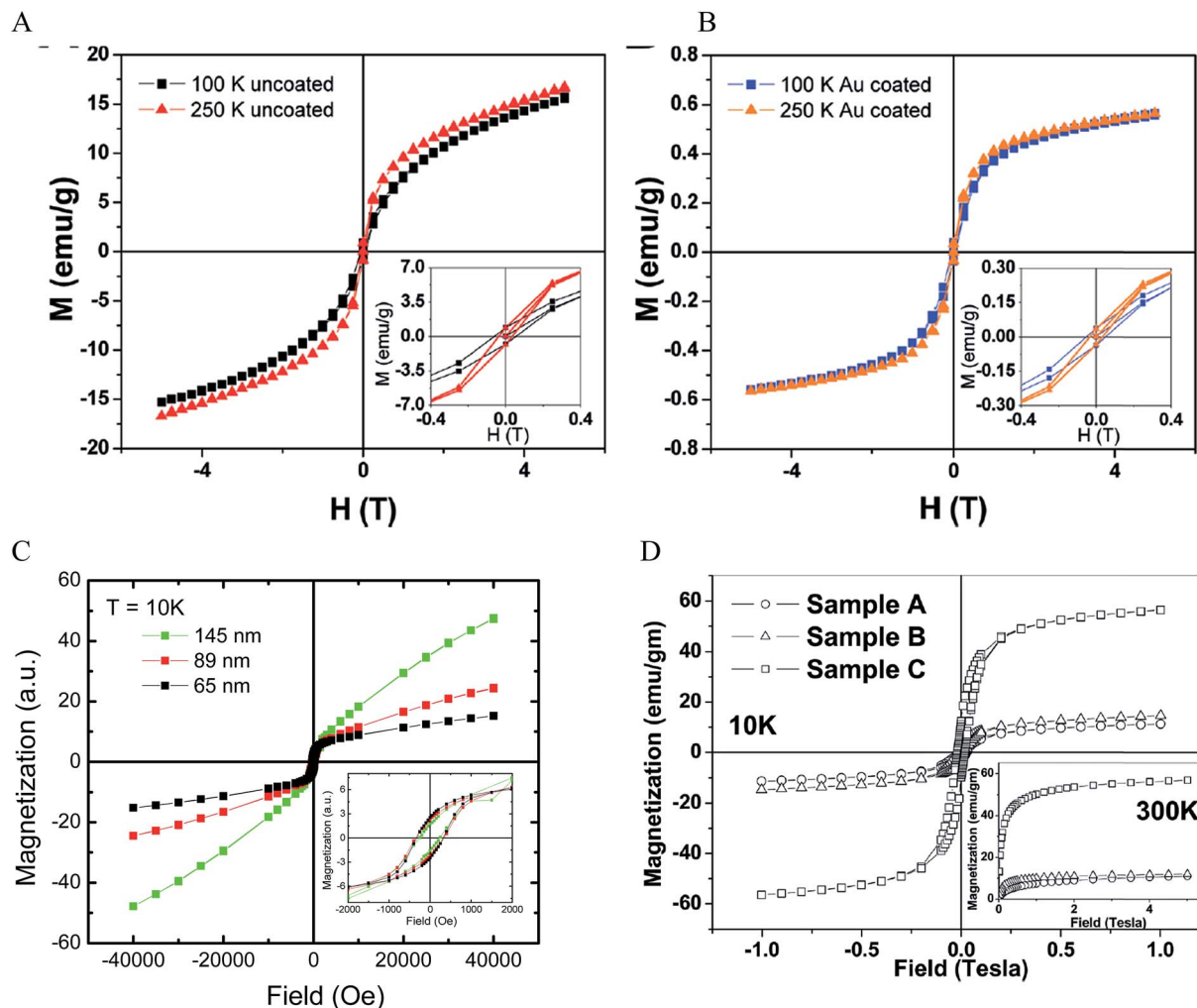
Fig. 6 Magnetic properties of IO–Au core–shell NPs. (A and B) Magnetization as a function of applied field at 100 K and 250 K for uncoated and Au coated tetra-cubic IO NPs. Reprinted with permission from ref. 69. Copyright (2009) American Chemical Society. (C) Magnetization as a function of applied field at 10 K for IO–Au core–shell nanopopcorns of three different sizes. Reprinted with permission from ref. 72. Copyright (2016) American Chemical Society. (D) Magnetization as a function of applied field at 10 K and 300 K for bare IO NPs (sample A), IO–Au core–shell NPs with low Au (sample B) and high Au (sample C). Reprinted with permission from ref. 46. Copyright (2011) American Chemical Society.
