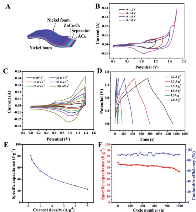
Fig. 6 (A) A schematic of the \text{ZnCo}_2\text{O}_4 //AC quasi-solid-state asymmetric supercapacitor. (B) CV curves obtained at different potential windows. (C) The CV curves obtained at various scan rates. (D) The GCD attributed to some irreversible reactions occurring in the potential curves under different current densities. (E) The specific capacitance of the device as a function of current density. (F) The cycling performance and the corresponding Coulomb efficiency at 0.5 \text{ A g}^{-1} .
