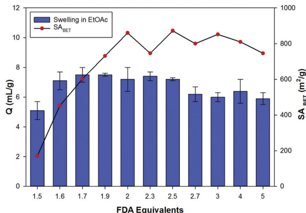
Fig. 3 Variation of the apparent BET surface area ( S_{\text{BET}} ) and swellability ( Q ) in ethyl acetate, for the toluene derived HCPs.
