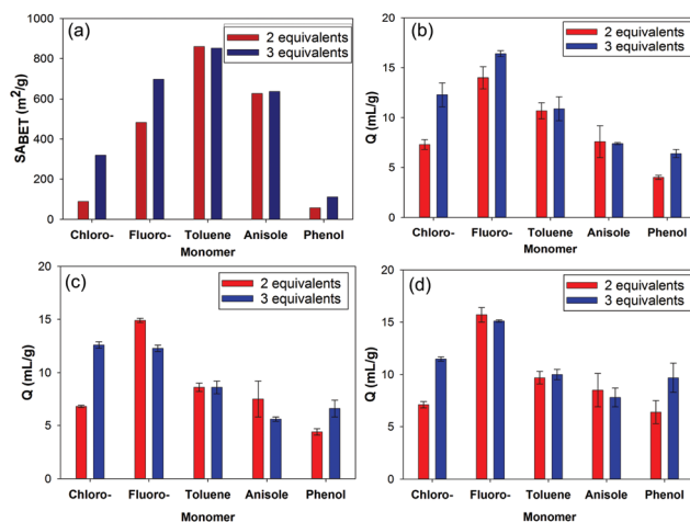
Fig. 4 (a) Apparent S_{\text{BET}} and swellability ( Q ) in; (b) triethylamine, (c) ethyl acetate, and (d) DMF for the HCPs prepared using 2 equivalents and 3 equivalents of FDA as crosslinker.
