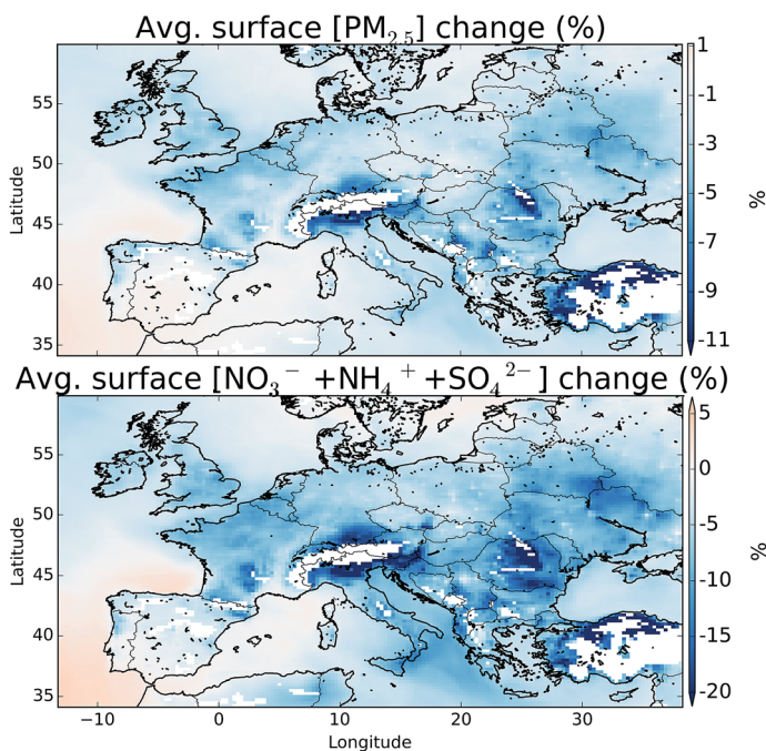
Fig. 12 Percentage difference in boundary layer surface ( >900\text{ hPa} ) total fine particulate matter (below 2.5\text{ microns} , PM 2.5 ), and the sulfate (SO 4 2- ), ammonia (NH 4 + ), and nitrate (NO 3 - ) mode between the simulation with halogens ("HAL") and without ("NOHAL"). Maximum values on the PM 2.5 and SO 4 2- + NH 4 + + NO 3 - plots are -21.1 and 34.9\% . Plotted regions are restricted to those with surface pressures greater than 900\text{ hPa} to remove larger influences at clean mountain top sites.
