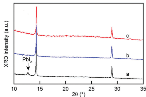
Fig. 6 XRD patterns of a MABr : \text{PbI}_2 solution with a molar ratio of either 1 : 1 in air (a) and an Ar-filled glovebox (b) or 1.2 : 1 in air (c); the down arrow indicates the position of the \text{PbI}_2 peak. Adapted from ref. 53 Copyright 2015, American Chemical Society.
