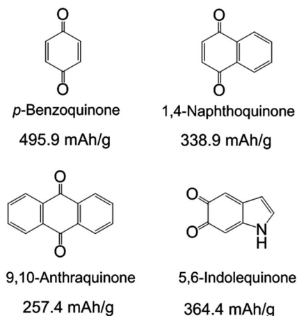
Scheme 1 Molecular structures and the corresponding theoretical capacity of p -benzoquinone, 1,4-naphthoquinone, 9,10-anthraquinone and 5,6-indolequinone. The theoretical capacities are calculated based on the redox reactions of carbonyl groups in the molecules.
