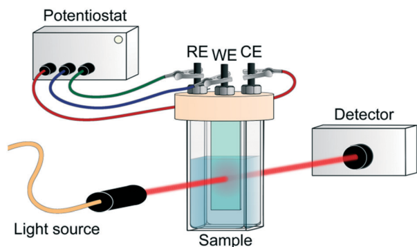
Fig. 5 Scheme of SEC experiment. RE, WE and CE refer to reference, working and counter electrode, respectively.
