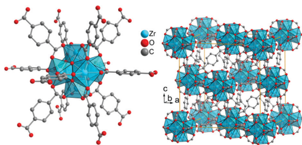
Fig. 9 Structure of zirconium terephthalate UiO-66Zr. The SBU is a hexanuclear and octahedral cluster of six edge-sharing ZrO_8 square antiprisms, which is connected to 12 neighboring SBUs in a face-centered cubic (fcc) packing arrangement. The structure was drawn from deposited cif-files under CCDC 837796 (UiO-66). 81
