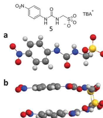
Fig. 7 Single crystal X-ray structure of (a) compound 5 which was shows (b) dimer formation through urea-anion hydrogen bond formation. The TBA counter cation and second sulfonate urea anion have been omitted for clarity where necessary. Nitrogen atoms blue, hydrogen atoms white, carbon atoms grey, oxygen atoms red, sulphur atoms yellow and fluoride atoms green. Crystals were obtained by slow evaporation of a chloroform solution containing 5 .
