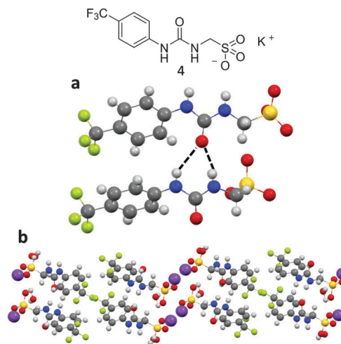
Fig. 6 Single crystal X-ray structure of compound 4 which was shows (a) hydrogen bonded self-association through syn -urea stacking and (b) the formation of hydrophobic and hydrophilic regions. The potassium counter cation and associated water molecules have been omitted for clarity where necessary. Nitrogen atoms blue, hydrogen atoms white, carbon atoms grey, oxygen atoms red, potassium atoms purple, sulphur atoms yellow and fluoride atoms green. Crystals were obtained by slow evaporation of the pyridinium intermediate of 1 in water with approximately one equivalent of potassium hydroxide.
