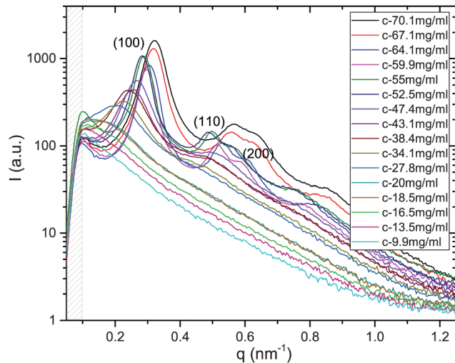
Fig. 2 X-ray scattering spectra plotted for the whole range of studied concentrations in the case of M13-PEG5k at I_s = 10 mM. For the dense rod packings (from C = 70.1 to 52.5 \text{mg mL}^{-1} ), the (100), (110) and (200) Bragg reflections are the hallmark of a 2D positional hexagonal ordering. At intermediate virus concentrations (between C = 47.4 and C = 20 \text{mg mL}^{-1} ), a broad (100) peak is evidenced, characteristic of liquid-like order. 11 Because at too low wavevector q , this structure factor peak is out of our accessible range for concentration C below 18.5 \text{mg mL}^{-1} . The gray dashed area indicates the unphysical region of the spectra near the beam stop.
